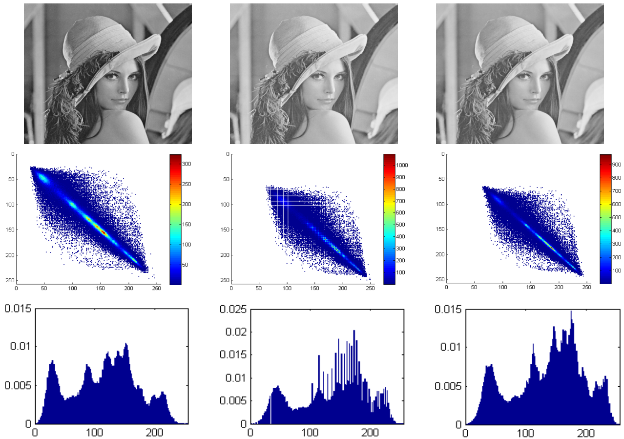
Fig. 2. The first row from left to right contains the original, CCE and ACE (CE here is Gamma Correction with g 0.6) images. The second row gives their corresponding GLCM (x and y-axes give gray values and colorbar gives the number of co-occurrence). The third row shows the corresponding normalized gray value histograms (x-axis is Gray value and y-axis is the probability of occurrence) of the images.
