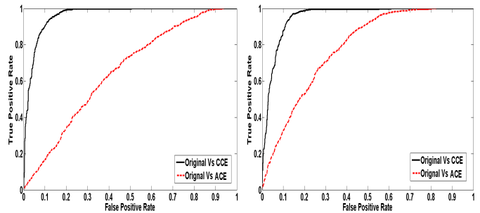
Fig. 3. ROC curve for detection of CE for original Vs CCE and original Vs ACE using CE detector proposed in [7] for Gamma Correction (left) and Histogram Stretching (right)
